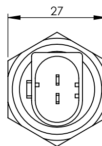
VIEW/VISTA A
