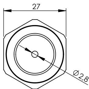
VIEW/VISTA B
