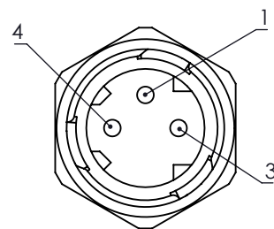
VIEW/VISTA A
