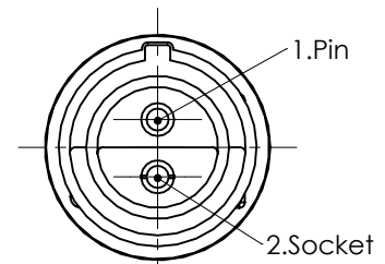
VIEW/VISTA A
