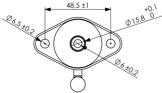
VIEW/VISTA A
