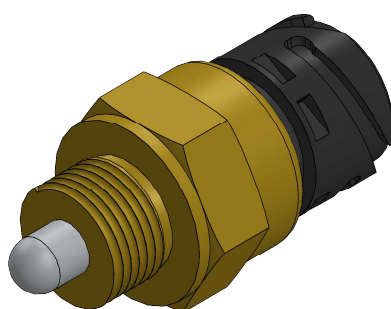
VIEW/VISTA A
