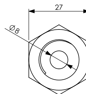
VIEW/VISTA B
