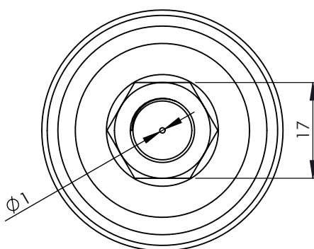
VIEW/VISTA A
