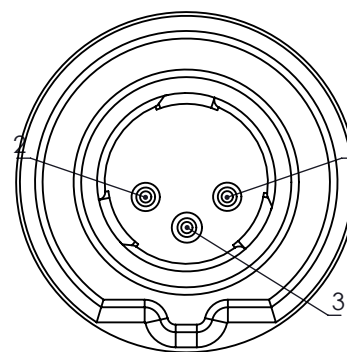
VIEW/VISTA B
