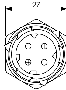
VIEW/VISTA B
