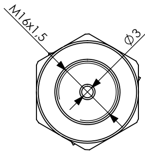
VIEW/VISTA A
