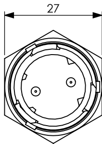
VIEW/VISTA A
