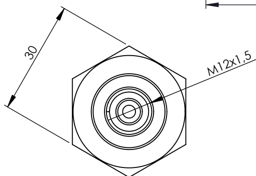
VIEW/VISTA B
