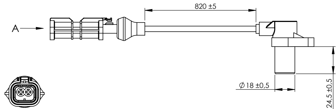
VIEW/VISTA A
