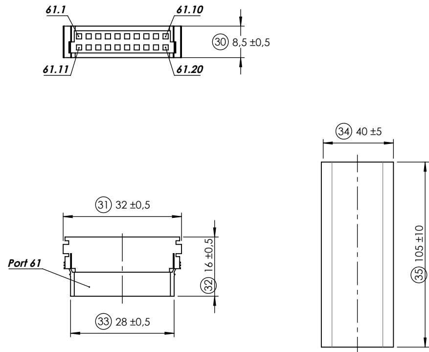
Scale / Escala 1 : 1 Protective tube included / Tubo protector incluido
