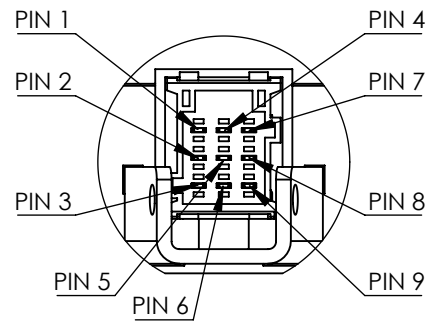
DETAIL/DETALLE A
