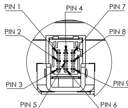
DETAIL/DETALLE A
