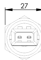
VIEW/VISTA A
