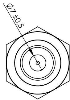
VIEW/VISTA A
