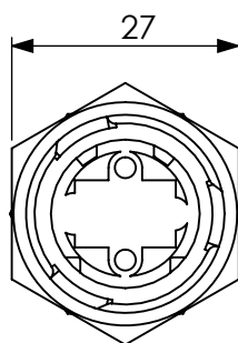
VIEW/VISTA A
